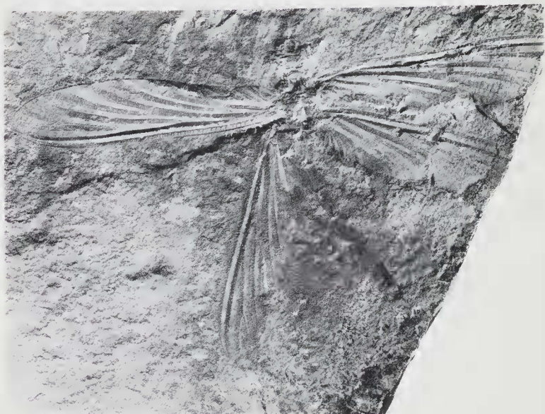
Figure 3. Protoreisma directum , n.sp. Photograph of paratype, MCZ 5182a, Permian of Oklahoma. Length of fore wing, 32 mm.
